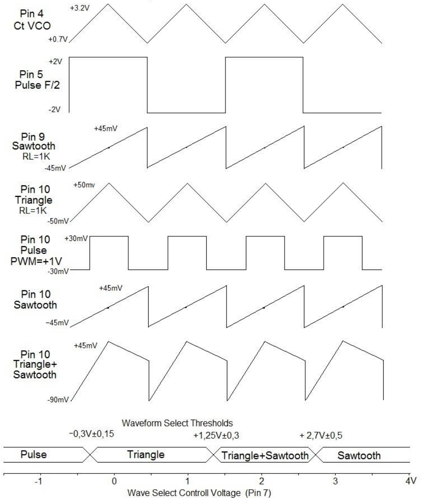
Fig.2 Wave select control voltages and thresholds
